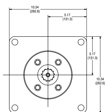
VIEW B-B
